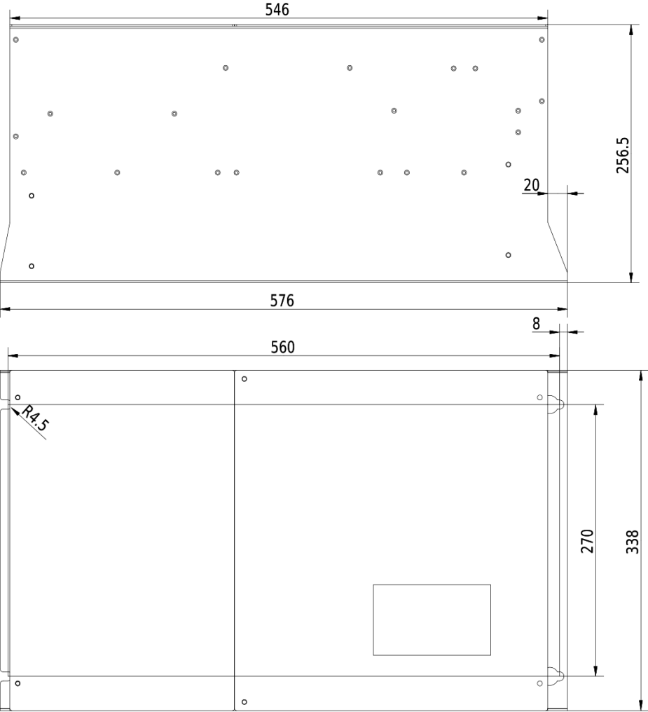
Dimensional drawing V800 - 75kW 4T0750
