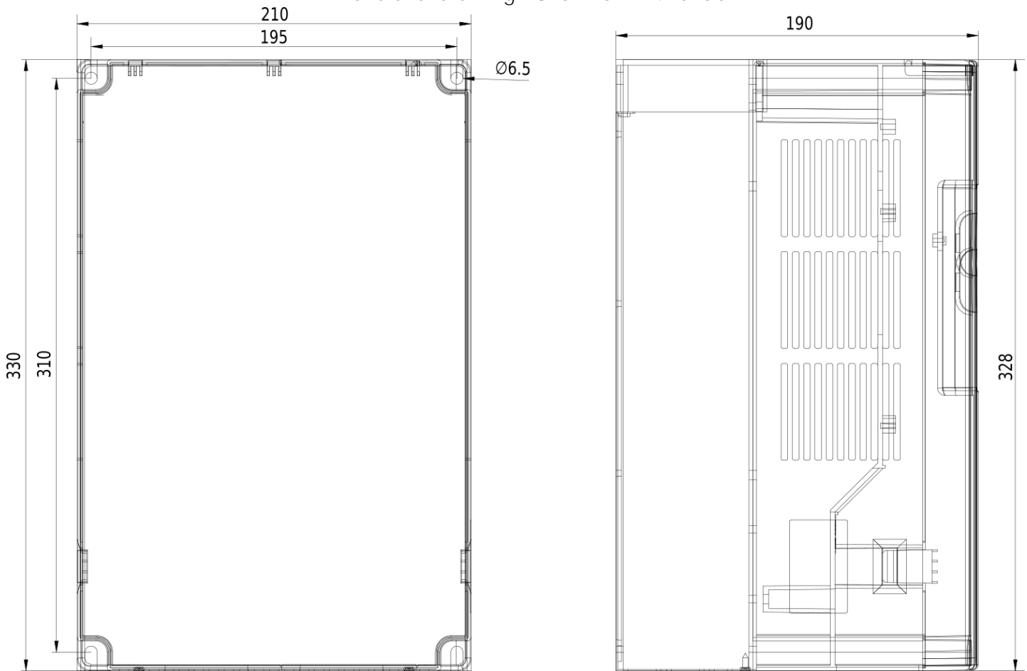
Dimensional drawing V810 - 15kW 4T0150
